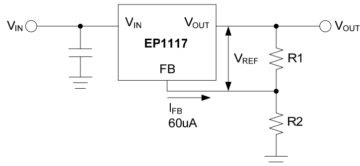
Figure 1-Basic Adjustable Regulator
